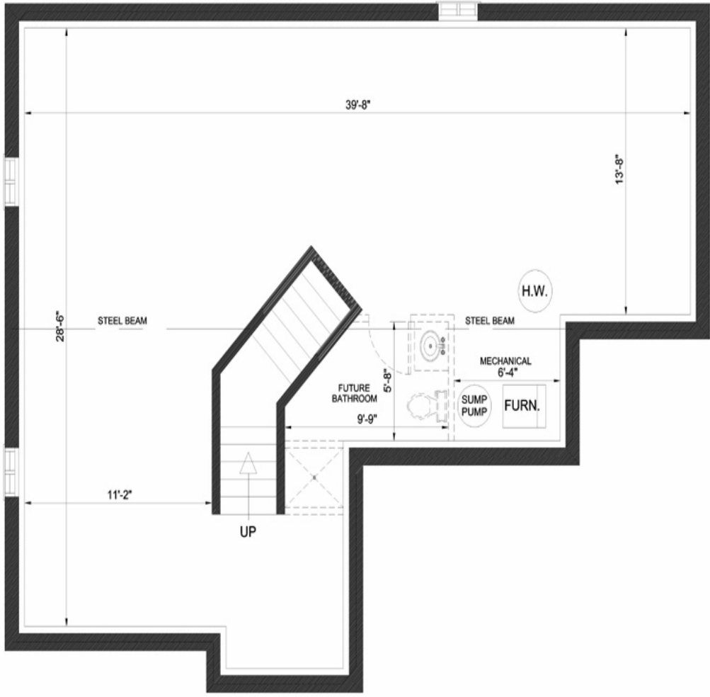
BASEMENT PLAN
