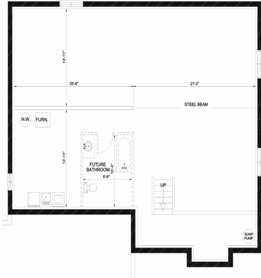
BASEMENT PLAN
