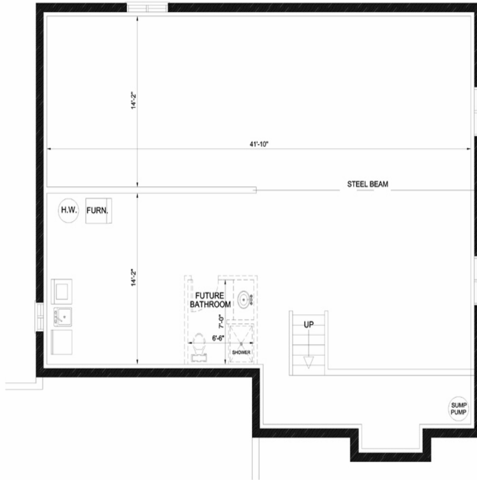
BASEMENT PLAN
